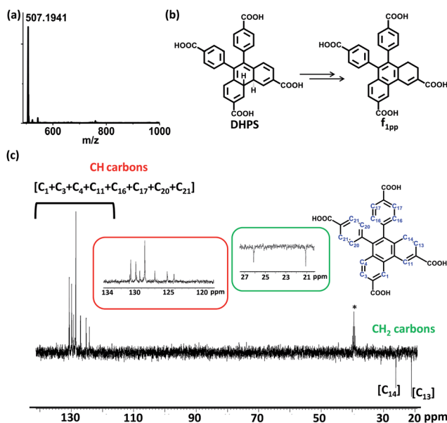
Fig. 3 (a) The ESI-MS of f_{1pp} in negative ion mode, (b) chemical transformation of DHPS to f_{1pp} , and (c) the DEPT spectrum of f_{1pp} in \text{CD}_3\text{OD} (insets show zoomed in regions (120–134 and 21–27 ppm) and the f_{1pp} structure with designated -\text{CH} and -\text{CH}_2 carbons, *signifies the \text{DMSO}-d_6 peak).
