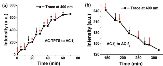
Fig. 5 (a) and (b) show the emission intensity of AC (0.9 wt%) conjugated with TPTS ( 10^{-4} \text{ M} ) ( l = 1 \text{ cm} , \lambda_{exc} = 350 \text{ nm} , water) followed at 400 nm under light (red arrows, 254 nm irradiation) and dark conditions (black arrows) for various times ((a) AC-TPTS to AC-f 1 , (b) AC-f 1 to AC-f 2 ).
