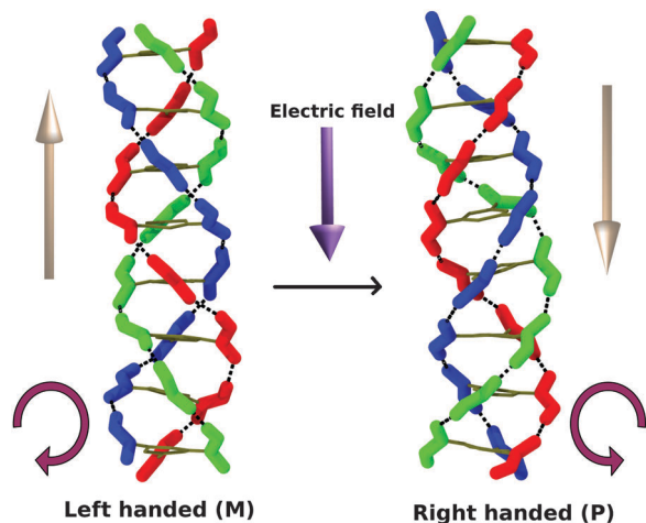
Fig. 4 Snapshot of a stack from MD simulations of the LC phase illustrating the reversal of chirality upon application of an electric field. In the initial geometry (left), H-bonded helices are twisted in the clockwise direction and the macrodipole points up. Amides present in each H-bonded helix are colored differently. Application of an electric field in the direction opposite to that of the macrodipole reverses the handedness i.e. , the helical twist turns counter-clockwise.
