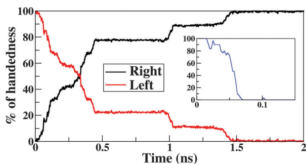
Fig. 5 Change in handedness of BTA stacks in the LC phase with time. The ordinate is the fraction of dihedrals ( C_{Ar}-C_{Ar}-C-O ) that are left-handed. See Fig. S3 (ESI † ) for dihedral definition. An electric field of magnitude 0.2 \text{ V \AA}^{-1} was applied at a temperature of 400 K at t = 0 . The inset shows the same for an arbitrarily chosen stack. Results for all stacks are shown in Fig. S4a (ESI † ).
