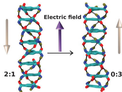
Fig. 3 Snapshot of one stack from MD simulations of the LC phase at 400 K. The change from an asymmetric (2:1) dipole configuration to a symmetric (0:3) one, upon application of the electric field ( \vec{E} = 0.2 \text{ V \AA}^{-1} ), is seen. The macrodipole moment is indicated by the brown arrow.
