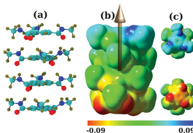
Fig. 1 (a) Optimized geometry of the tetramer of N,N,N' -tris(methyl)-benzene-1,3,5-tricarboxamide at the B3LYP/6-311+g(d,p)//B3LYP/cc-pVTZ level of theory. Side chains are methyl groups. Color: C – cyan; O – red; N – blue; H – tan. (b) Isosurface of electrostatic potential at 0.004 e bohr -3 . Arrow indicates the macrodipole. (c) Top and bottom views of a tetrameric stack.
