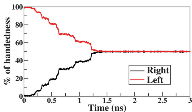
Fig. 7 Transformation of an enantiomerically pure (left-handed) system into a racemic mixture upon the application of an electric field. At t = 0 , all the stacks are left-handed (100%) which yield equal amounts of left-(50%) and right-(50%) handed stacks upon the application of an electric field.
