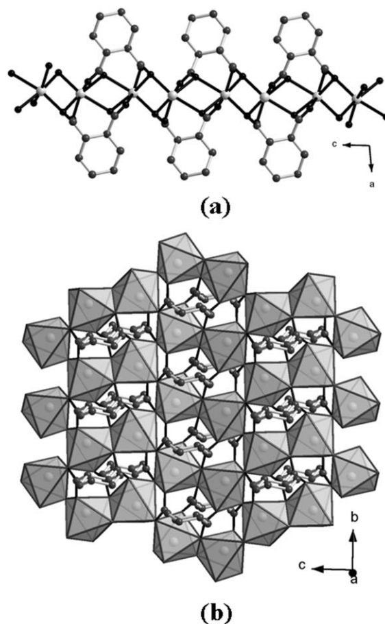
Fig. 10 (a) Structure of [\text{Cd}(\text{C}_8\text{H}_{10}\text{O}_4)] , IX along the b axis and (b) structure of IX , showing the infinite M–O–M linkage.
