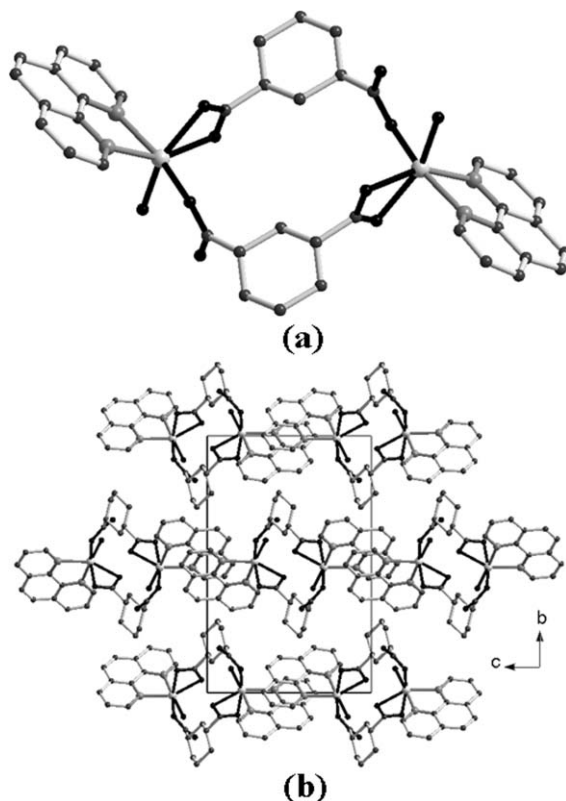
Fig. 9 (a) Structure of [\text{Mn}(\text{H}_2\text{O})(\text{C}_8\text{H}_{10}\text{O}_4)(\text{C}_{12}\text{H}_8\text{N}_2)] , VIII and (b) packing arrangement in VIII viewed along the a axis.
