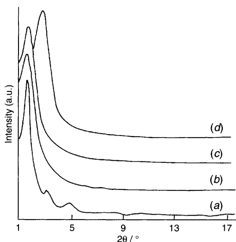
Fig. 1 XRD patterns of the mesophases of silica: (a) obtained with hexadecylamine (water content, x = 4.4 mol); (b) with hexadecylamine (water content, x = 1.33 mol); (c) hexagonal phase obtained by the calcination of (a), and (d) hexagonal phase obtained with octylamine
