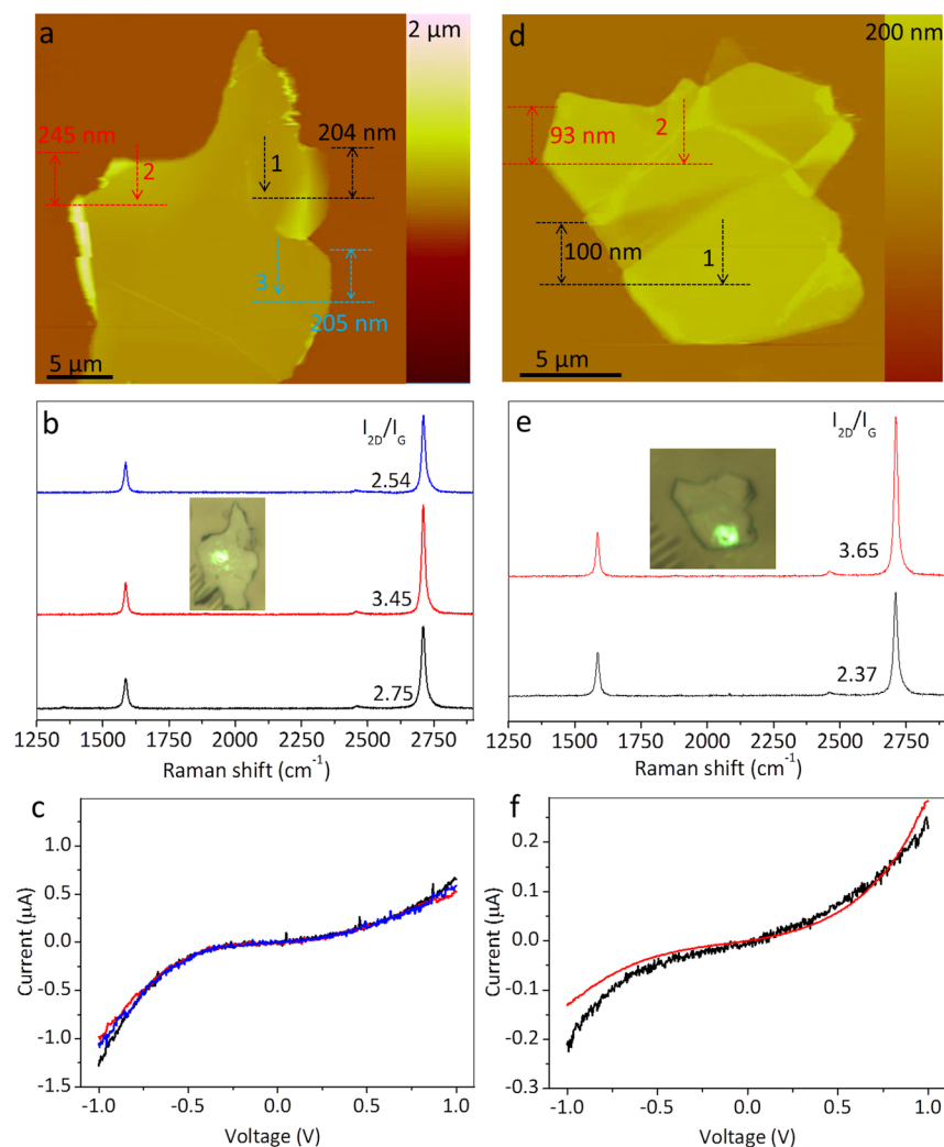
Figure 2. Raman and C-AFM measurements on T-SLG. (a,d) AFM topography of typical T-SLG flakes. Arrows marked 1 (black), 2 (red), and 3 (blue) indicate the spots where Raman and I–V measurements have been made. The flake thicknesses are shown adjacent to the spots. (b,e) Raman spectra from the corresponding regions with its I_{2D}/I_G values. Insets show optical micrographs of the T-SLG flakes with incident Raman beam. (c,f) I–V characteristics of graphene multilayers measured using conducting AFM at the designated spots.
