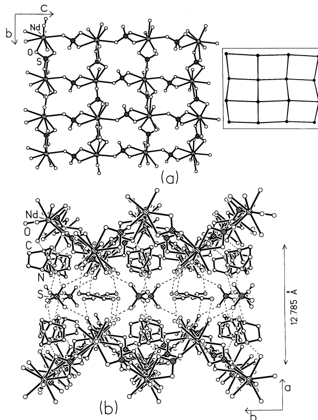
Fig. 10 (a) Top view of the layer parallel to the bc -plane in V , formed by joining the NdO 9 polyhedra and SO 4 tetrahedra. The inset shows the (4, 4) net sheet formed by the joining of the metal centers. (b) The stacking of the alternate inorganic layers and the layer formed by the ethylenediamine molecules, sulfate ions and the interstitial water molecules, along the a -axis of the unit cell. The protonated DABCO molecules reside in the crest and trough regions of the inorganic layer. Dotted lines represent hydrogen-bond interactions. Note the wavelike pattern of the inorganic layers.
