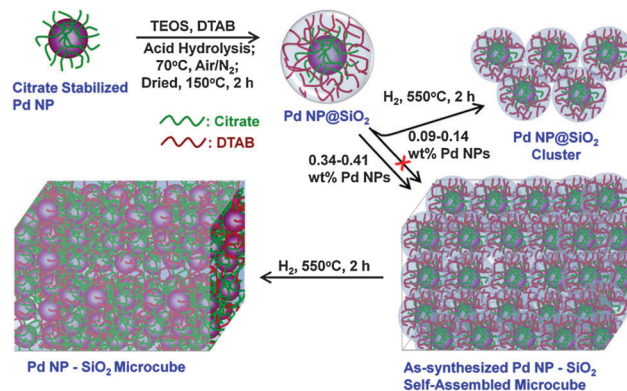
Fig. 2 Schematic illustration of the formation process of Pd-SiO 2 microcubes.
