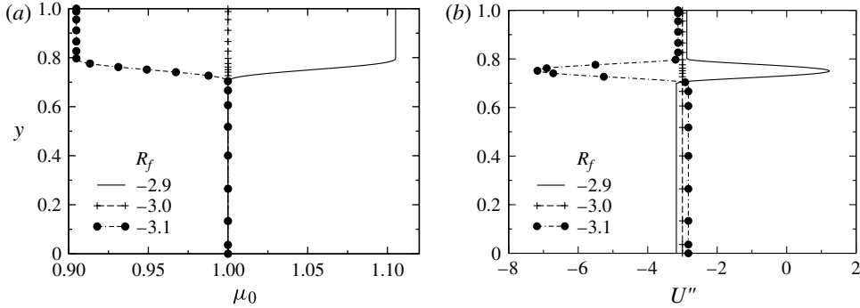
FIGURE 2. Basic steady-state profiles of (a) viscosity (b) second derivative of the streamwise velocity, for different values of R_f . The other parameters are chosen as h = 0.7 , q = 0.1 , Re = 200 and R_s = 3 .
